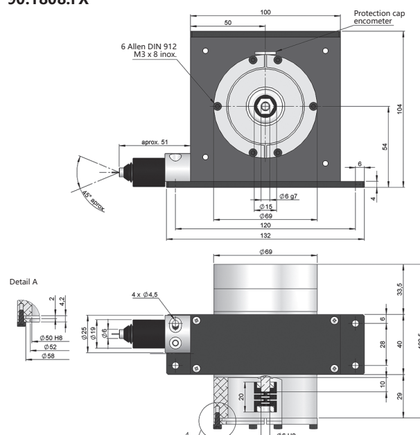
Drawing 90.1808.FX with flexible accessory, standard bell synchro and coupling type 1
