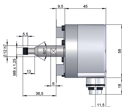
Drawing shaft type 1, anti-rotation system type 4, connection type 2
