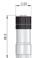
Female connector 95.0007152
